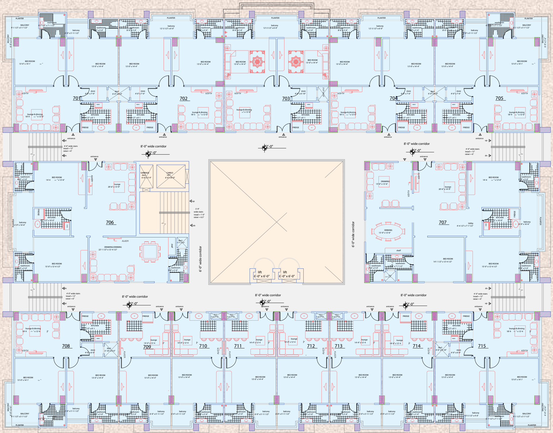
7TH floor at level of +72'-0"
