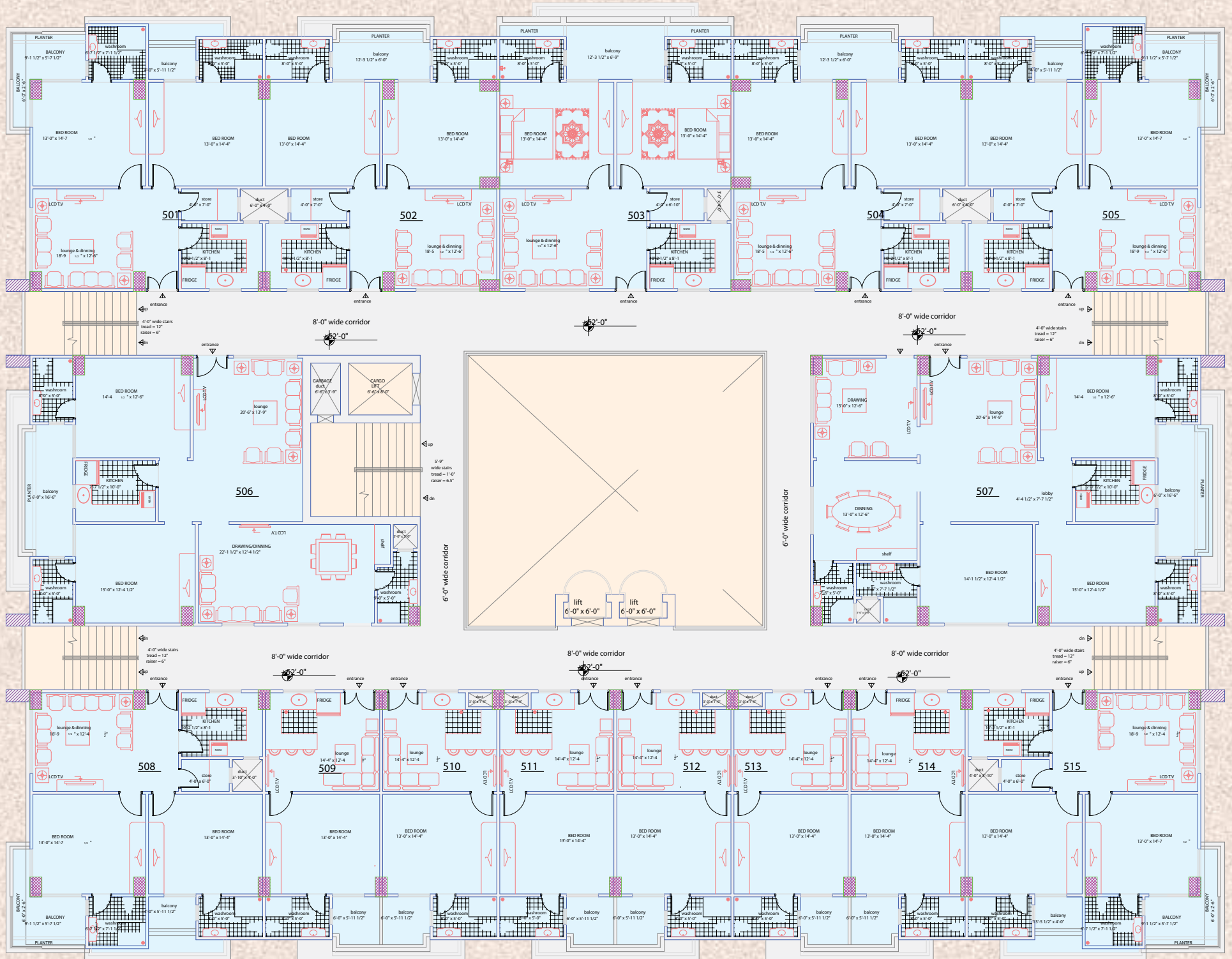
5TH floor at level of +52'-0"
