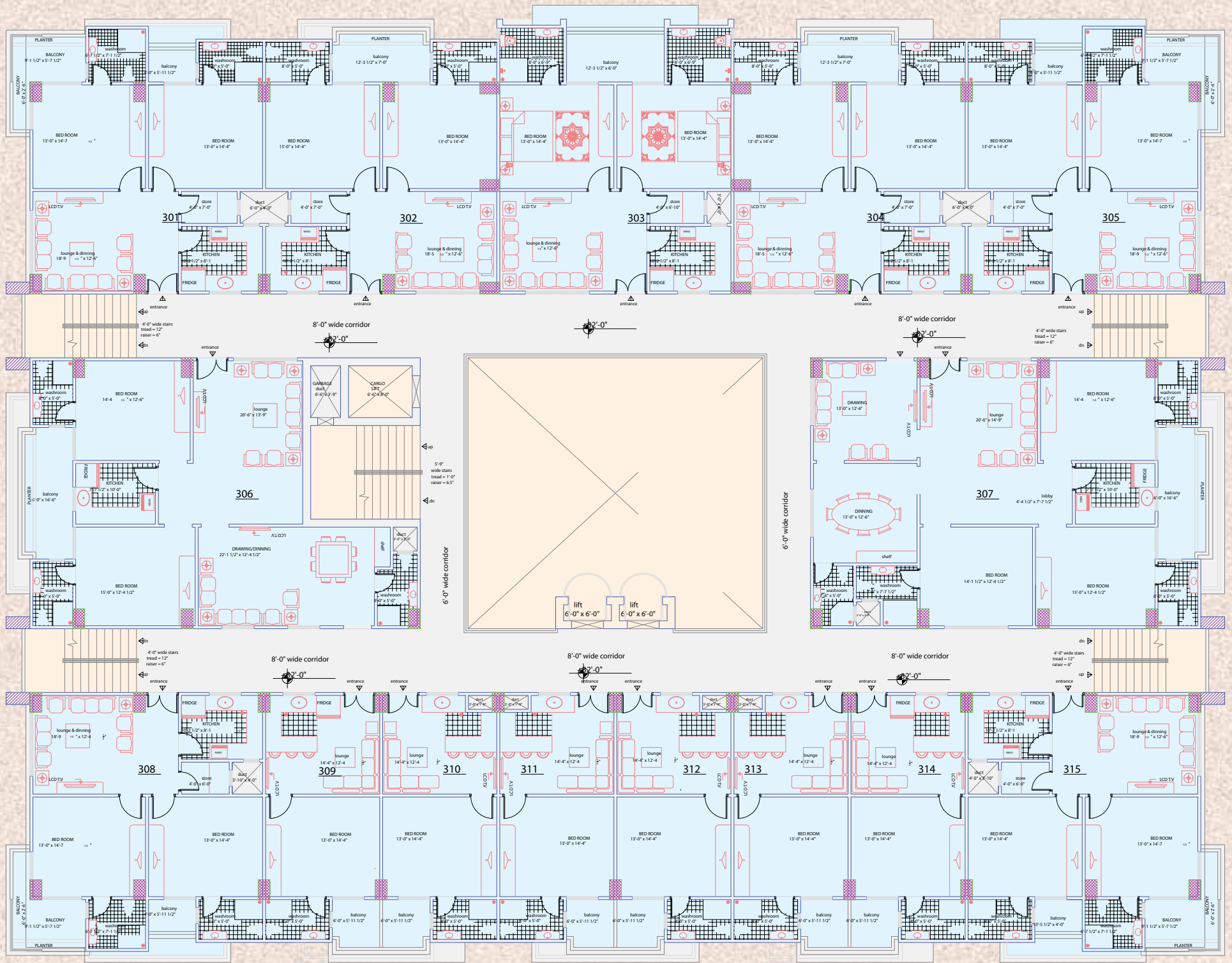
3rd floor at level of +32'-0"
