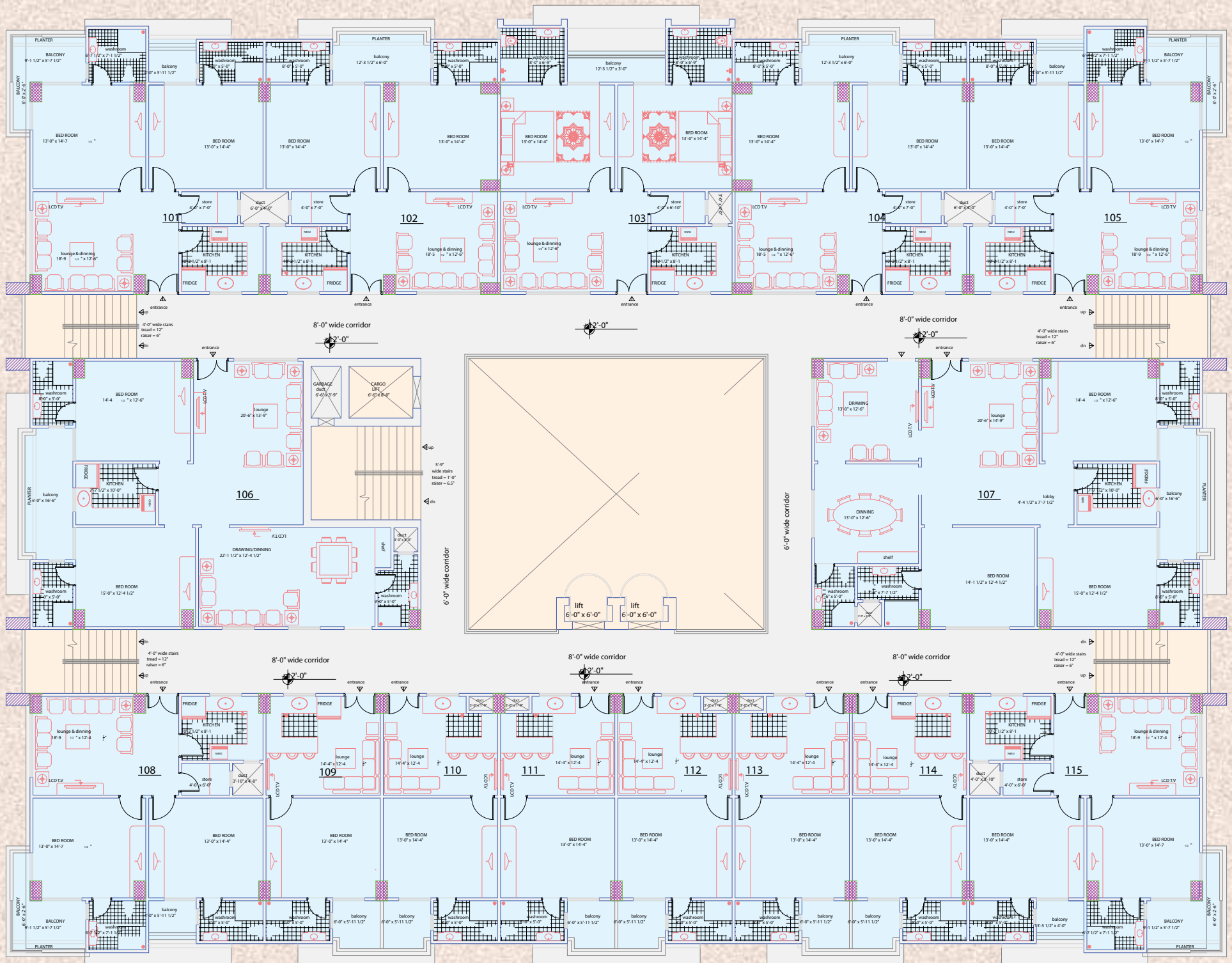
1st floor at level of +12'-0"
