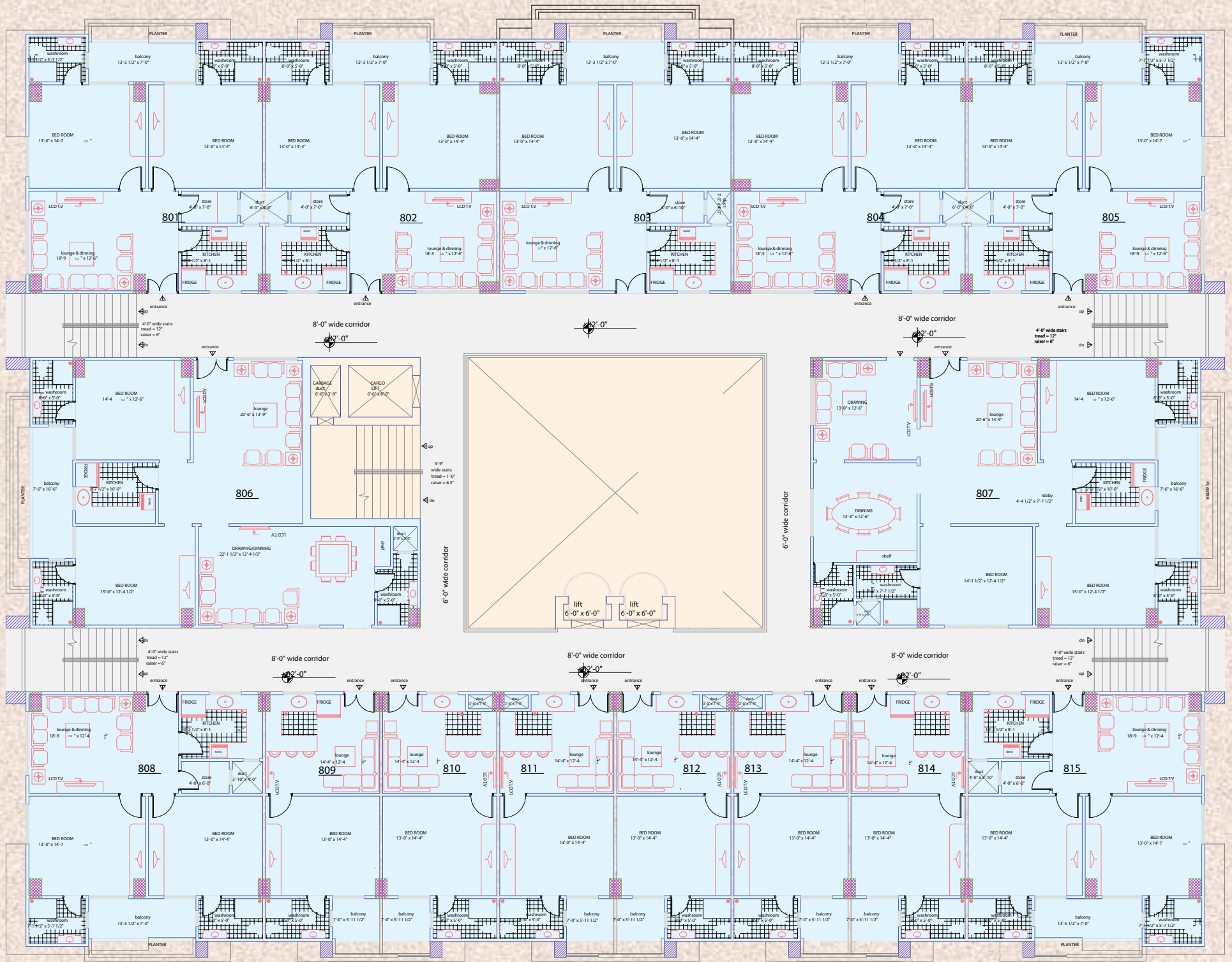
8TH floor at level of +82'-0"
