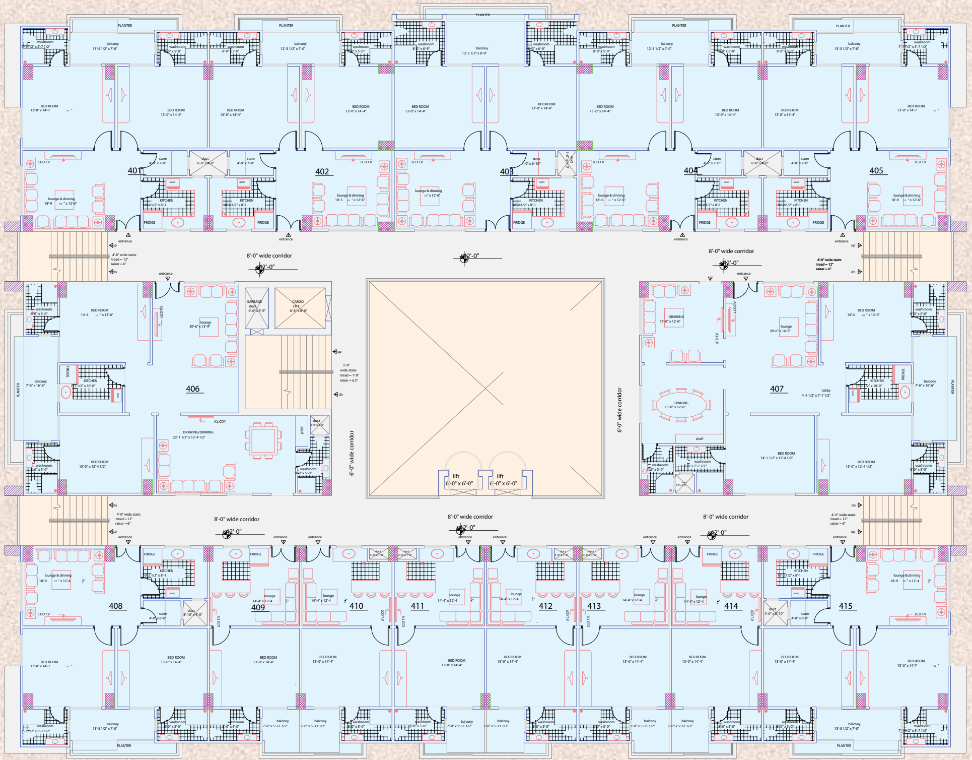
4TH floor at level of +42'-0"
